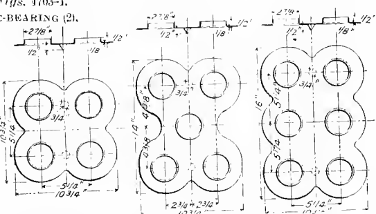
Figs. 4710-4715. STEEL OR MALLEABLE-IRON SPRING-SEATS AND CAPS. For Cars of 40,000, 50,000 and 60,000 lbs. capacity respectively.
